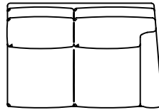
47-48-2/2-LAF Left Arm Facing Loveseat Overall: H36 W56 D38 Inside: W48 D21 1/2 Seat: H20 Arm: H25 1/2
