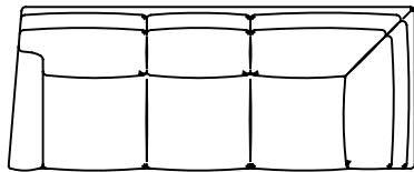
49-70-3/3-LAF Left Arm Facing Corner Sofa Overall: H36 W94 D38 Inside: W69 1/2 D21 1/2 Seat: H20 Arm: H25 1/2
