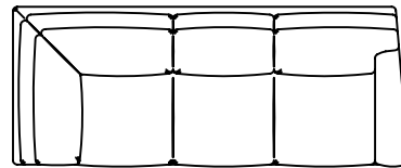
49-70-3/3-LAF Left Arm Facing Corner Sofa Overall: H36 W94 D38 Inside: W69 1/2 D21 1/2 Seat: H20 Arm: H25 1/2
