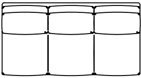
48-72-3/3-A Armless Sofa Overall: H36 W72 D38 Inside: W72 D21 1/2 Seat: H20
