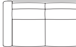
4727-LAF McGrath Left Arm Facing Loveseat Overall: H32 W62 D37 Seat: W54½ D22 Seat: H19 Arm: H25½
