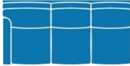
LEFT ARM FACING SOFA 33 - 72 - 3/3 - LAF OVERALL: H37½ W77 D38 INSIDE: W72 D21½ SEAT: H20 ARM: H26
