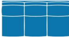
ARMLESS SOFA 33 - 72 - 3/3 - A OVERALL: H37½ W72 D38 INSIDE: W72 D21½ SEAT: H20
