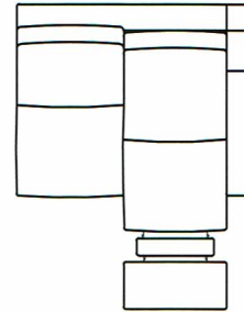
11207-43-RAF-INC-MR Salon Right Arm Facing Motorized Inclining Loveseat (Reclining Position) Overall: H42½ W54 D46½ Inside: W48 D21 Seat: H21½ Arm: H25½ Depth Fully Reclined: 71
