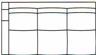
11208-43-LAF-INC-MR Salon Left Arm Facing Motorized Inclining Sofa (Closed Position) Overall: H42½ W79 D46½ Inside: W72 D21 Seat: H21½ Arm: H25½
