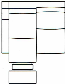
11207-43-LAF-INC-MR Salon Left Arm Facing Motorized Inclining Loveseat (Reclining Position) Overall: H42½ W54 D46½ Inside: W48 D21 Seat: H21½ Arm: H25½ Depth Fully Reclined: 71
